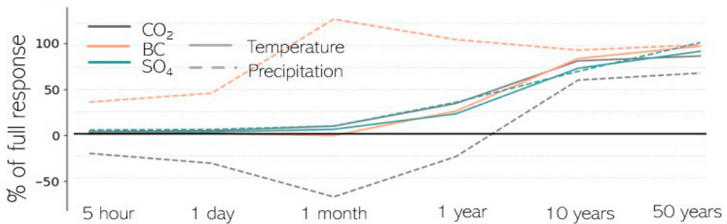
FIG. 7. Schematic of time scales of climate responses to \text{CO}_2 , BC, and \text{SO}_4 , focusing on the main changes to temperature, precipitation, and high and low clouds. Vertical lines illustrate changes from the baseline (black) vertical temperature profile. Note that temperature profiles are highly stylized, as are selected changes in high/low clouds and precipitation. (bottom) Model-average percentages at 100-yr (ERF normalized) response for chosen time periods.
