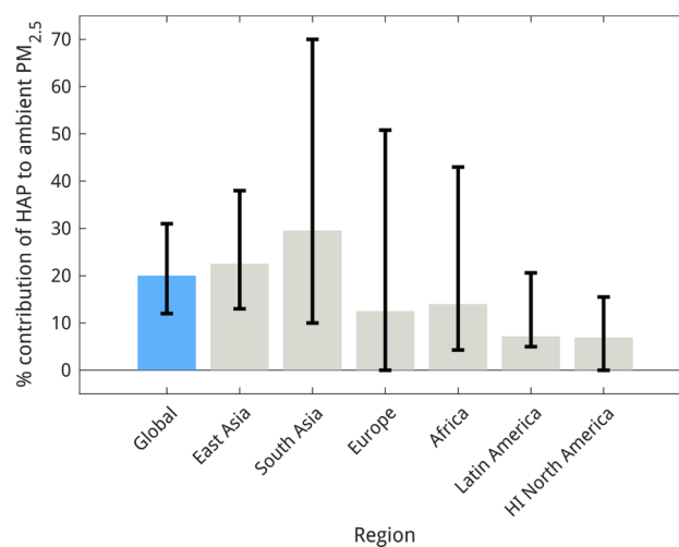
Fig. 3. The percentage of population-weighted exposure to ambient PM 2.5 due to solid fuel use in households. The bars indicate the median from the studies reviewed here, the whiskers range across the highest and lowest estimates.
