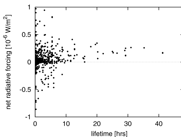
Figure 5. Instantaneous net radiative forcing of contrails relative to the contrail lifetime for winter and summer weather situations.
