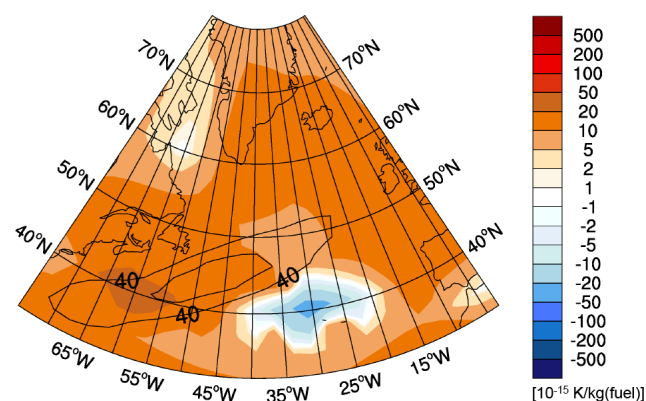
Figure 16. Merged climate change functions in 10^{-15} K per kilogram of fuel of aviation-induced total \text{NO}_x , contrail cirrus, and \text{H}_2\text{O} at 250 hPa exemplarily for weather situation S2 for an emission at 12:00 UTC.
