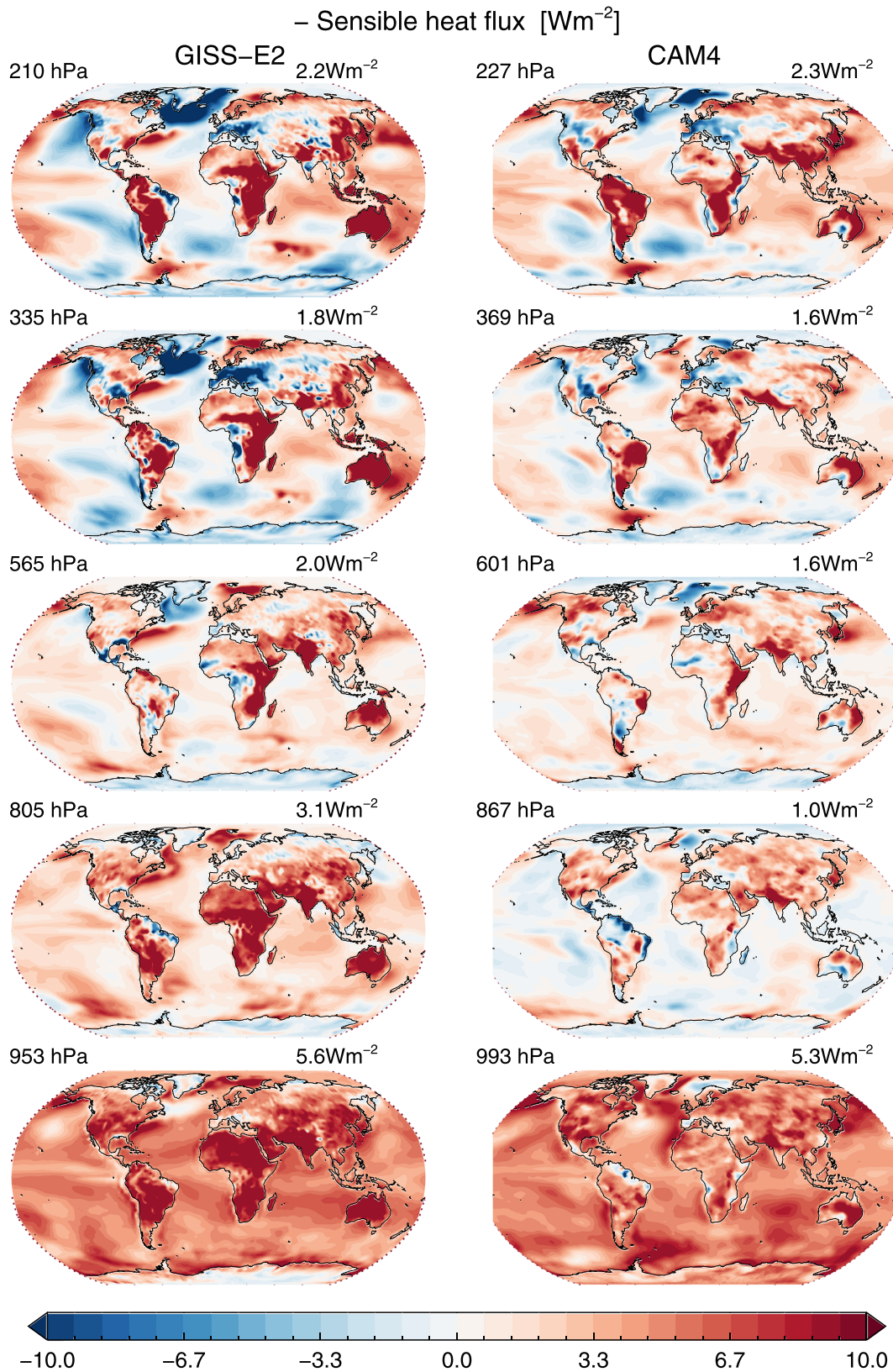
Figure 8. Annual mean change in surface sensible heat between five perturbed fSST runs and the baseline run. The BC injection height/layer for the perturbed run is specified in hPa, for GISS-E2 (left) and CAM4 (right).
