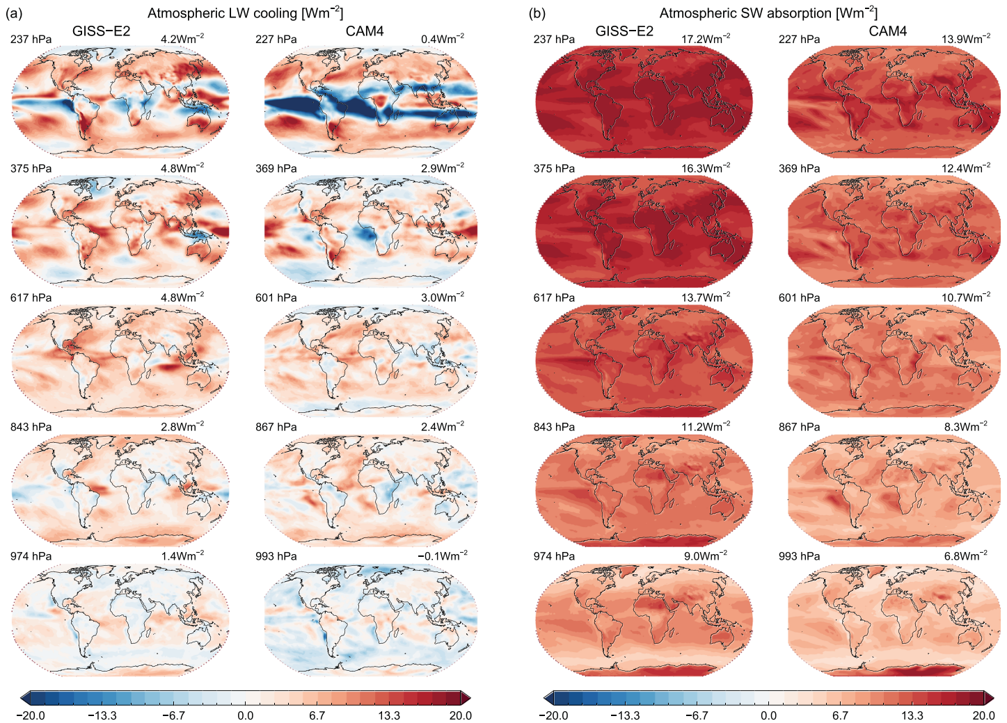
Figure 7. Annual mean change in (a) LW cooling and (b) SW absorption between five perturbed fSST runs and the baseline run (fast response). The BC injection height/layer for the perturbed run is specified in hPa, for GISS-E2 (left) and CAM4 (right).
