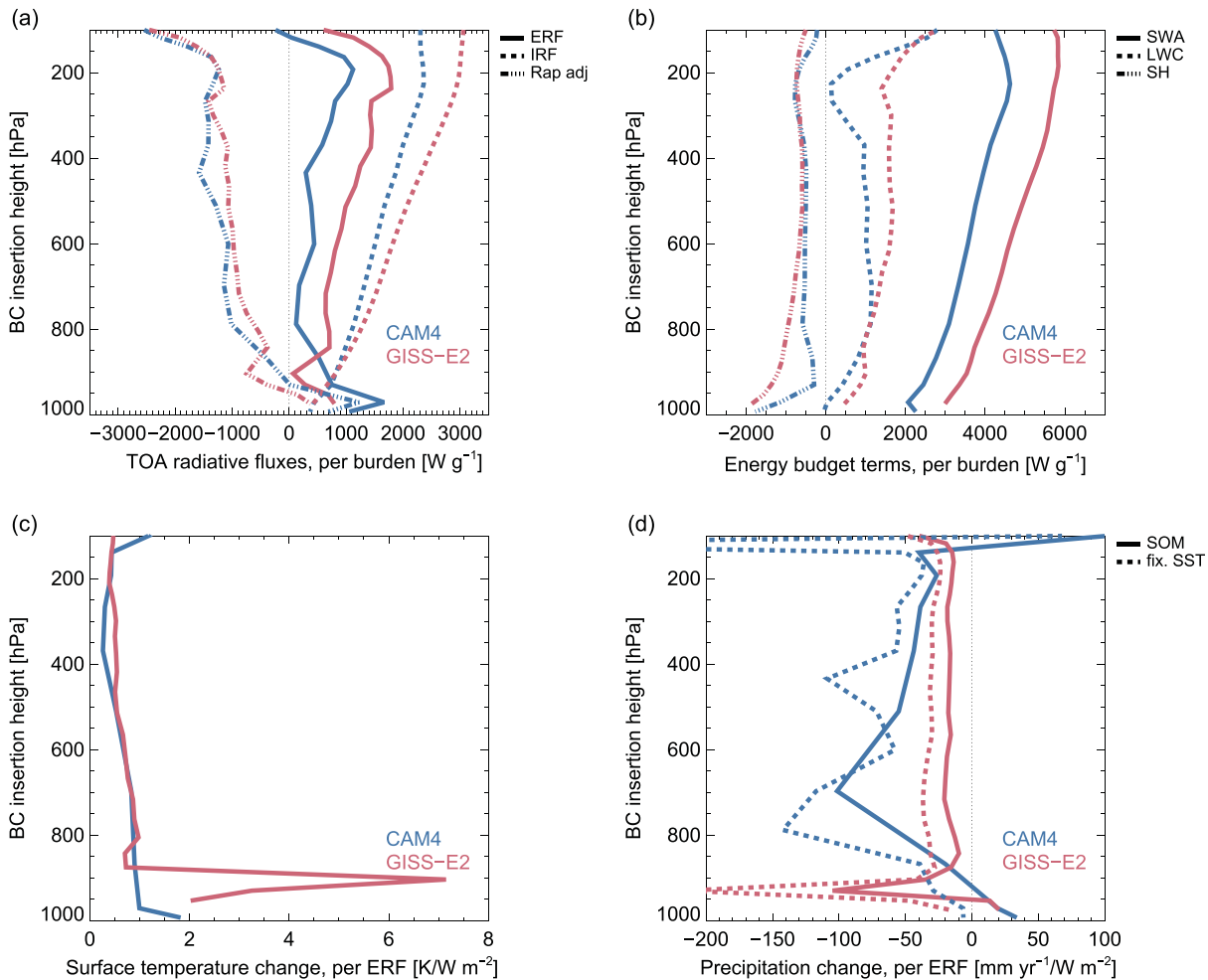
Figure 1. (a) Changes in the TOA radiative fluxes per burden for each layer of inserted BC in the fSST runs. The y-axis marks in the layer BC was inserted (in hPa). ERF is the net TOA flux (solid), IRF is the TOA direct radiative effect (dotted curve), and Rap adj is the rapid adjustment as the flux at TOA (striped-dotted). (b) SW absorption, (solid) LW cooling (dotted), and sensible heat flux (dotted-striped) for each BC layer in the fSST runs. (c) Surface temperature response per forcing for each BC layer in the SOM ocean runs ( K/Wm^{-2} ). (d) Precipitation change per forcing ( mm\ yr^{-1}/W\ m^{-2} ) for each BC layer in the fSST runs and the SOM runs, respectively.
