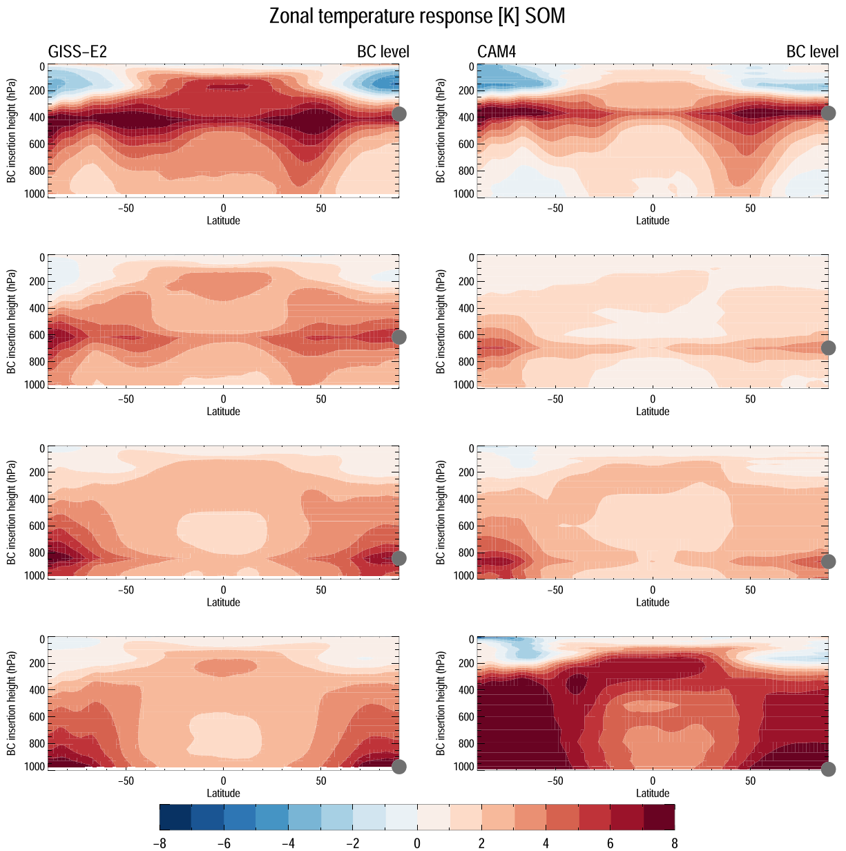
Figure 9. Zonal mean temperature change between four SOM runs and the baseline run for GISS-E2 (left column) and CAM4 (right column), for example, the total response (fast + slow). The gray dots indicate the BC insertion height.
