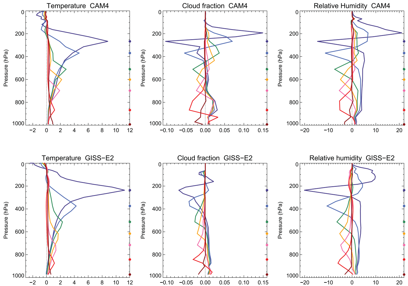
Figure 6. Changes in global mean temperature, relative humidity, and cloud fraction per height at seven selected perturbed fSST runs and the baseline run, in CAM4 (top) and GISS-E2 (bottom). The dots on the second y-axis represent the BC injection height for each experiment.
