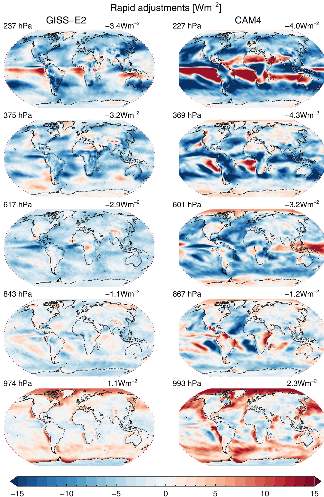
Figure 4. Annual mean change in the rapid adjustments between five perturbed fSST runs and the baseline run (fast response). The BC injection height/layer for the perturbed run is specified in hPa, for GISS-E2 (left) and CAM4 (right). Global mean change in rapid adjustments at TOA is given on top of each plot.
