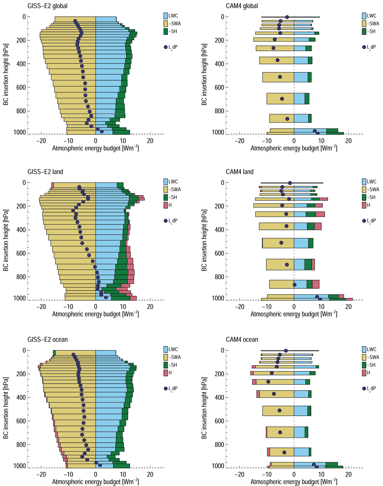
Figure 3. As in Figure 2, but for the total (fast + slow) response (SOM runs). Note that not all layers were perturbed for CAM4.
