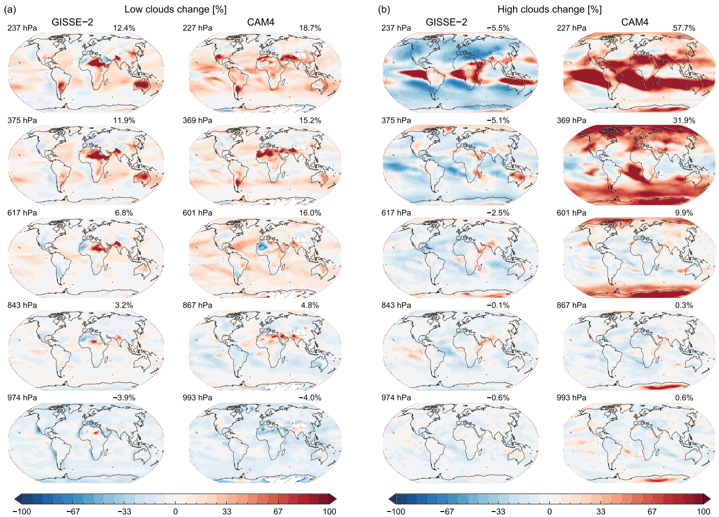
Figure 5. Annual mean relative change (%) in (a) low cloud fraction and (b) high cloud fraction between five perturbed fSST runs and the baseline run (fast response). The model layer with the added BC is specified in hPa, for GISS-E2 (left column) and CAM4 (right column).
