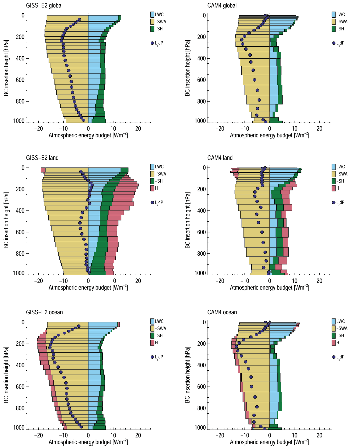
Figure 2. The atmospheric energy budget for each BC insertion for the fast-feedbacks (fSST runs) global average (top), land average (middle), and ocean average (bottom). Each bar represents one simulation (perturbation-baseline). The y-axis marks the altitude of the layer at which BC was inserted. LWC is the longwave cooling, SWA is the shortwave absorption, SH is the sensible heat flux, L_c is the latent heat of condensation, P is precipitation, and H is the dry static energy divergence. Note the sign convention, chosen so that positive changes imply a precipitation increase.
