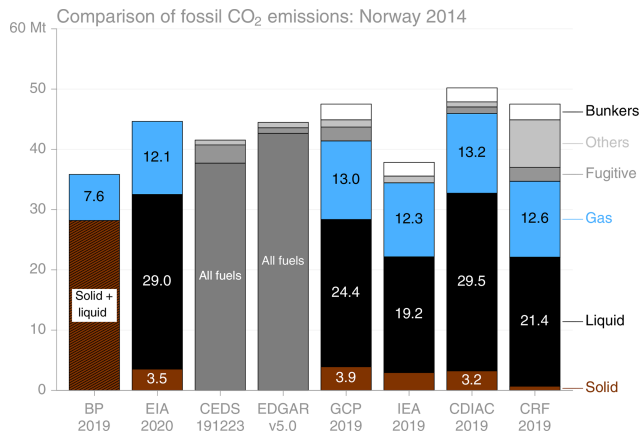
Figure 16. Comparison of fossil CO 2 emissions from eight sources for Norway.
