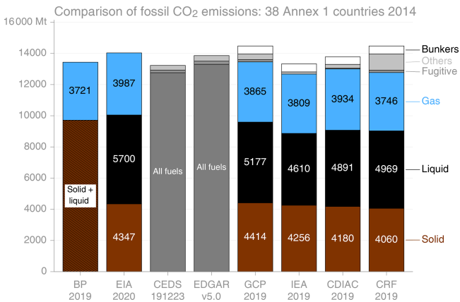
Figure 7. Comparison of fossil CO 2 emissions in most Annex 1 countries for the year 2014 from eight datasets. Smaller emitters (Cyprus, Israel, Liechtenstein, Malta) are excluded to increase the number of datasets in the comparison.
