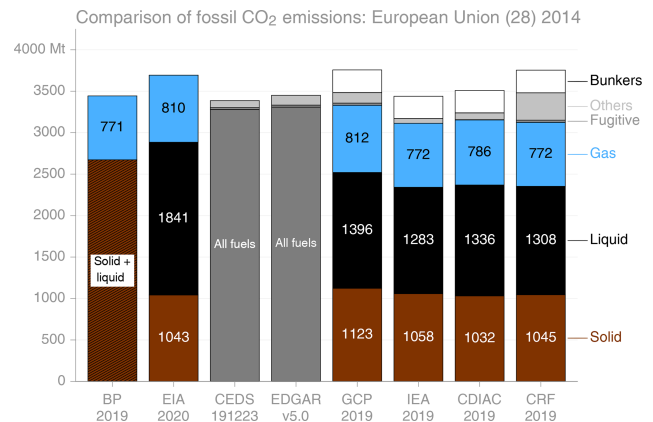
Figure 11. Comparison of fossil CO 2 emissions from eight sources for the European Union (28 members).
