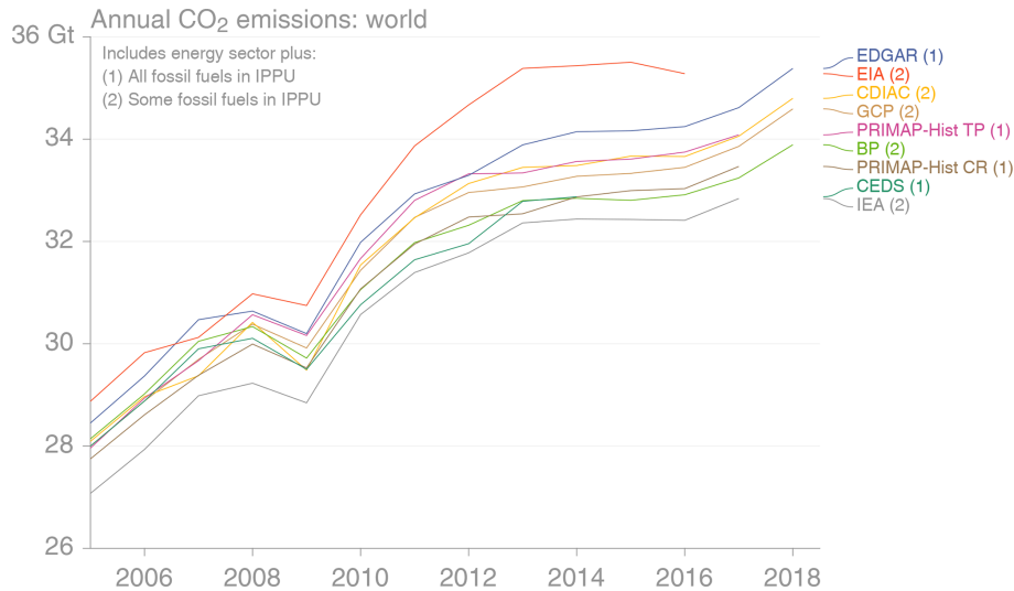
Figure 4. Annual global CO 2 emissions from various sources using similar system boundaries.
