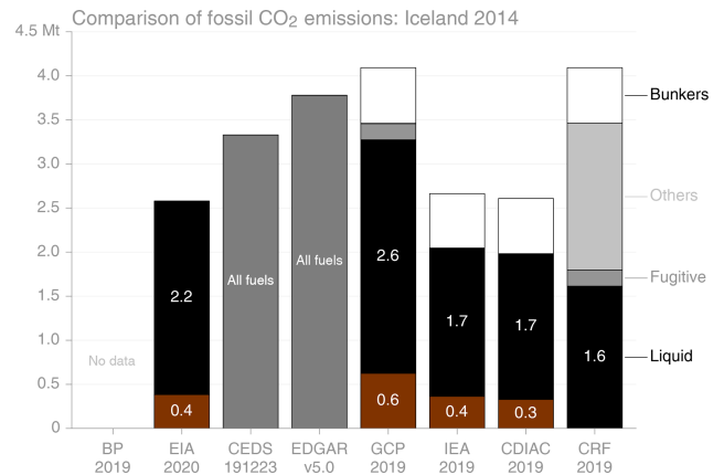
Figure 15. Comparison of fossil CO 2 emissions from six sources for Iceland.
