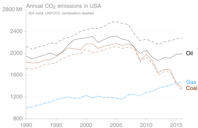
Figure 9. Comparison of emissions estimates for the USA from the IEA and UNFCCC.
