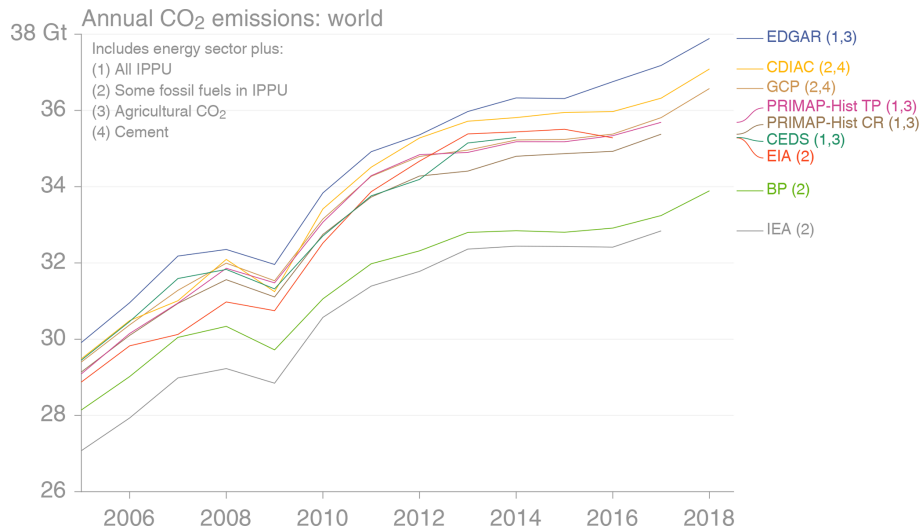
Figure 3. Annual global CO 2 emissions from various sources: total emissions. Sources: see Table 1.
