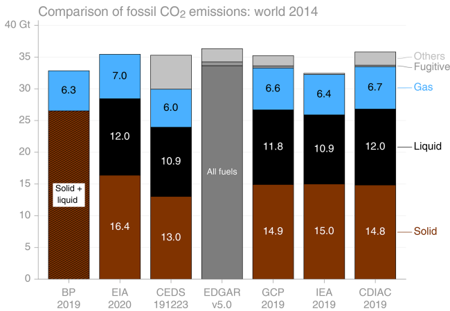
Figure 5. Comparison of global CO 2 emissions for the year 2014 from seven datasets, broken down by fuel type. BP and EDGAR do not report emissions by fuel type.
