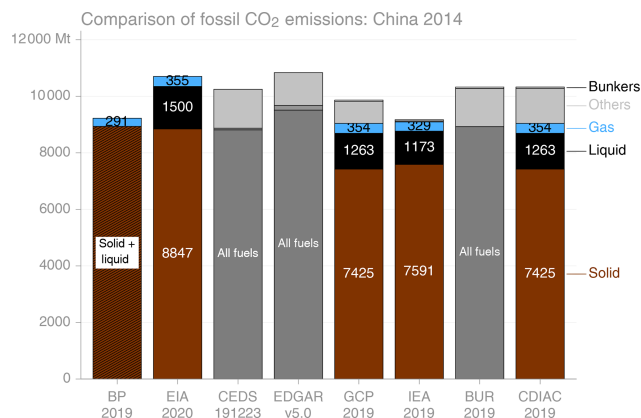
Figure 12. Comparison of fossil CO 2 emissions from seven sources for China.
