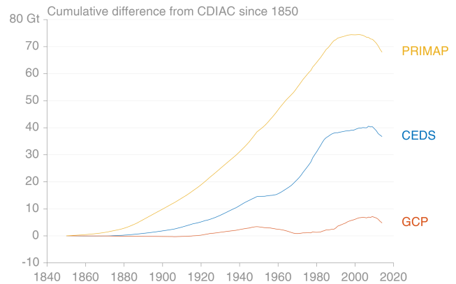
Figure 18. Difference of cumulative global CO 2 emissions from various datasets from those of CDIAC, starting in 1850.
