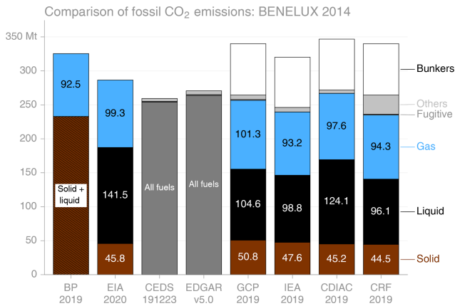
Figure 13. Comparison of fossil CO 2 emissions from seven sources for the Netherlands, Belgium, and Luxembourg.
