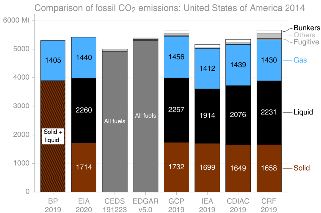
Figure 8. Comparison of CO 2 emissions estimates in the USA from eight datasets, 2014.
