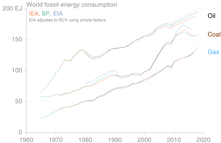
Figure 6. Global energy consumption estimates from three sources. The EIA reports energy production in gross calorific value (GCV), and this has been converted to net calorific value (NCV) using the standard factors of 0.9 for natural gas and 0.95 for oil and coal.
