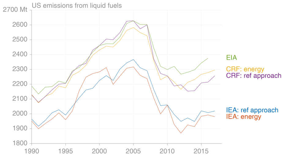
Figure 10. Comparison of estimates for CO 2 emissions from US liquid fuels, from the EIA, CRF (EPA), and the IEA.
