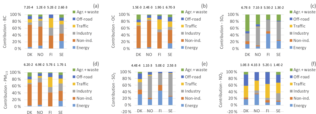
Figure 8. Population-weighted sectoral contributions of Finnish emissions on surface (a) BC, (b) OC, (c) SO 4 , (d) PM 2.5 , (e) SO 2 and (f) NO 2 over the Nordic countries. The labels above the bars show the absolute total contribution in \mu\text{g m}^{-3} from all the sectors in Finland.
