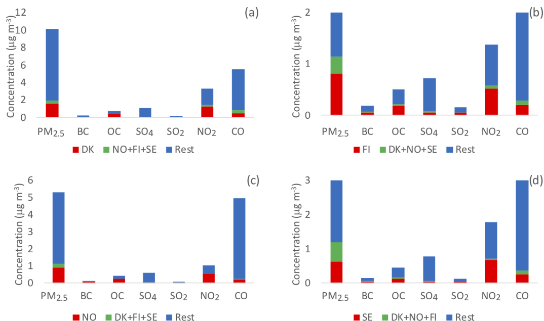
Figure 5. Absolute contributions of national, Scandinavian and other sources on the surface levels of major air pollutants over (a) Denmark, (b) Finland, (c) Norway and (d) Sweden. Note that CO concentrations are divided by 20 to scale with other pollutants.
