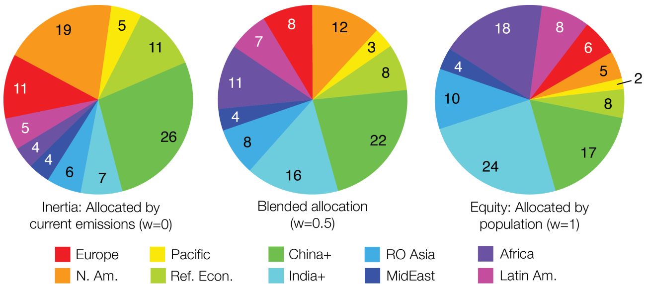
Figure 1: Sharing the carbon quota pie. Piecharts show shares of an available carbon quota allocated to 10 regions (Europe, North America, Pacific OECD, Reforming Economies, China+, India+, Rest of Asia, Middle East, Africa, Latin America) under three sharing principles based on Eq. (2), with sharing index w = 0, 0.5 and 1. Numbers give the percentage share of the global quota allocated to each region, summing to 100 for each piechart. Shares are calculated using Eq. (2) with emissions ( f_j ) averaged over last 5 years of data, and population ( p_j ) averaged over a 5-year period centred on the time at which world population reaches 9 billion. See SI Text 1 (Methods) for details.
