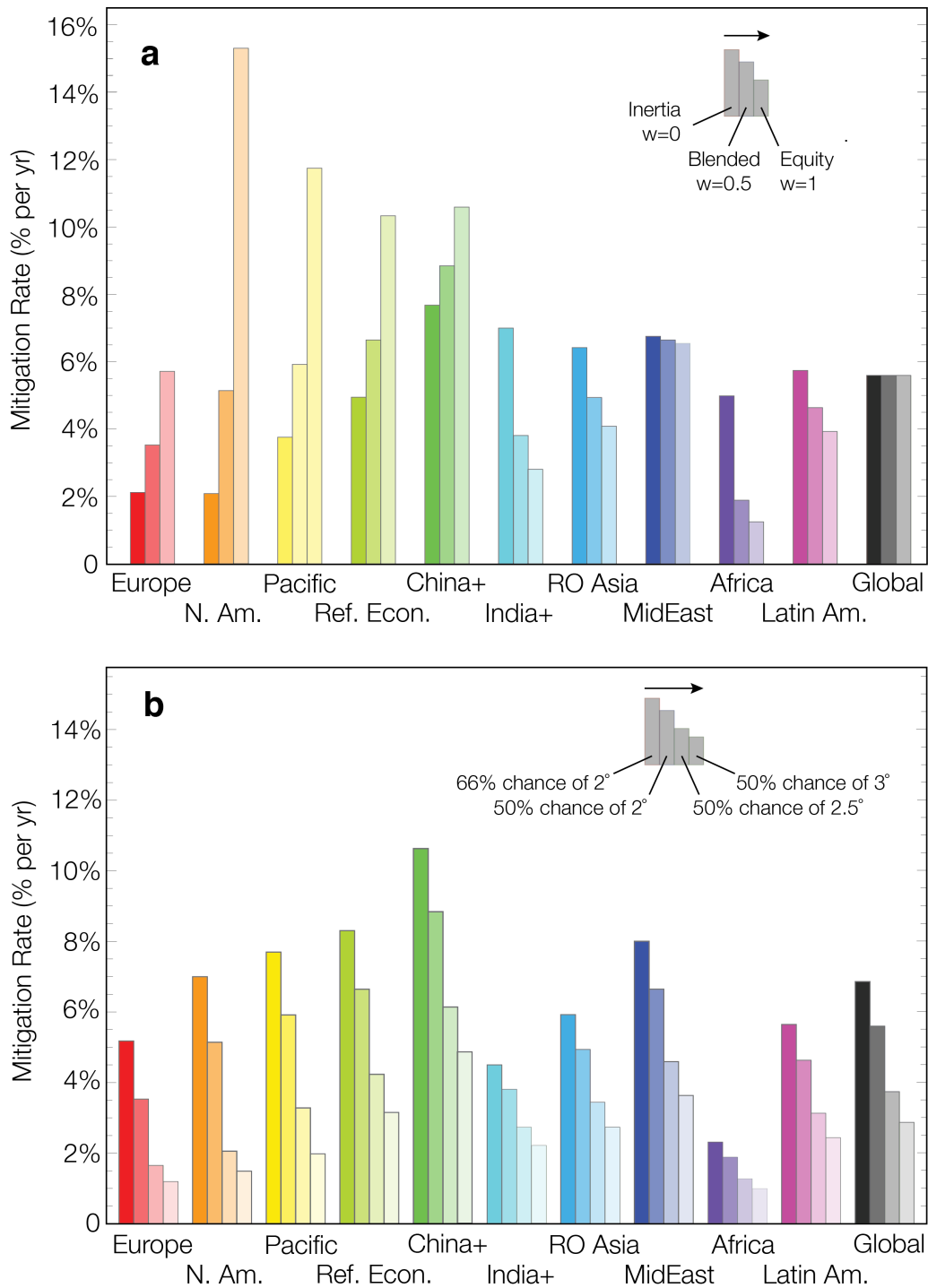
Figure 3: The dependence of the regional mitigation challenge on the sharing index ( w ) and the warming limit. Panel (a) shows mitigation rates for 10 regions and the world at w = 0, 0.5 and 1 . Available global FFI carbon quota from 2013 is Q^{\text{Avail}} = 1400 \text{ GtCO}_2 , corresponding to a 2-degree warming limit with 50% success probability. Panel (b) shows mitigation rates under a blended sharing principle ( w = 0.5 ) in four cases with (warming limit, success probability) equal to (2 degrees, 50%), (2.5 degrees, 50%), (3 degrees, 50%), (2 degrees, 66%). The available global FFI carbon quotas for these four cases are Q^{\text{Avail}} = 1400, 2300, 3200, 1100 \text{ GtCO}_2 , respectively 10 .
