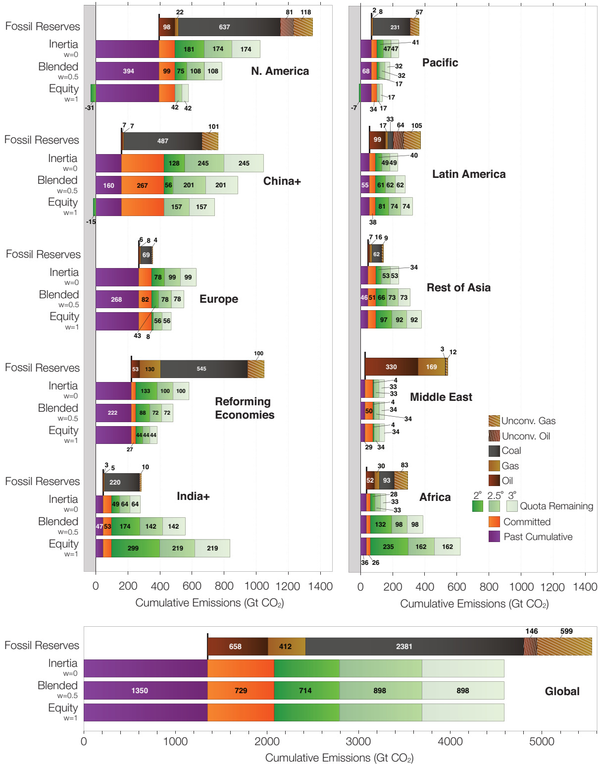
Figure 2: Quotas, cumulative committed emissions and fossil-fuel reserves. Past cumulative fossil-fuel CO 2 emissions (purple), future committed emissions 42,44 (orange) and available fossil-fuel carbon quotas to meet warming limits of 2, 2.5 and 3 degrees with 50% probability (green), for 10 regions and the world, under inertia, blended and equity sharing principles. Stacked bars are cumulative; numbers give the contribution of each increment in GtCO 2 . Negative increments are shown below the zero axis. Also shown are fossil-fuel reserves (coal, oil, gas, unconventional oil, unconventional gas) 12 .
