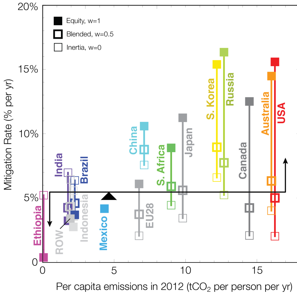
Figure 4: Distribution of the mitigation challenge among countries. Mitigation rates ( m ) for 14 countries and regions spanning the development spectrum and for the whole world, with sharing index w = 0 (open squares), w = 1 (filled squares) and w = 0.5 (half-open squares). Horizontal axis is 2012 per-capita fossil-fuel CO 2 emissions. Available global fossil-fuel carbon quota from 2013 is Q^{\text{Avail}} = 1400 \text{ GtCO}_2 , corresponding to a 2-degree warming limit with 50% success probability. With increasing equity in the sharing principle, the mitigation challenge increases for countries to the right of the point for the world (the pivot for the see-saw) and decreases for countries to the left. Mexico is so close to the pivot that symbols are indistinguishable.
